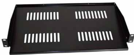
Shelf 1U or 2U, 300mm deep Part No.: SHELF1 = 1U shelf SHELF2 =2U shelf
