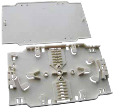
Splice tray lid and holder (Avaible in Beige or black) Part No.: TRAYBK = Tray black color TRAYBG = Tray beige color
